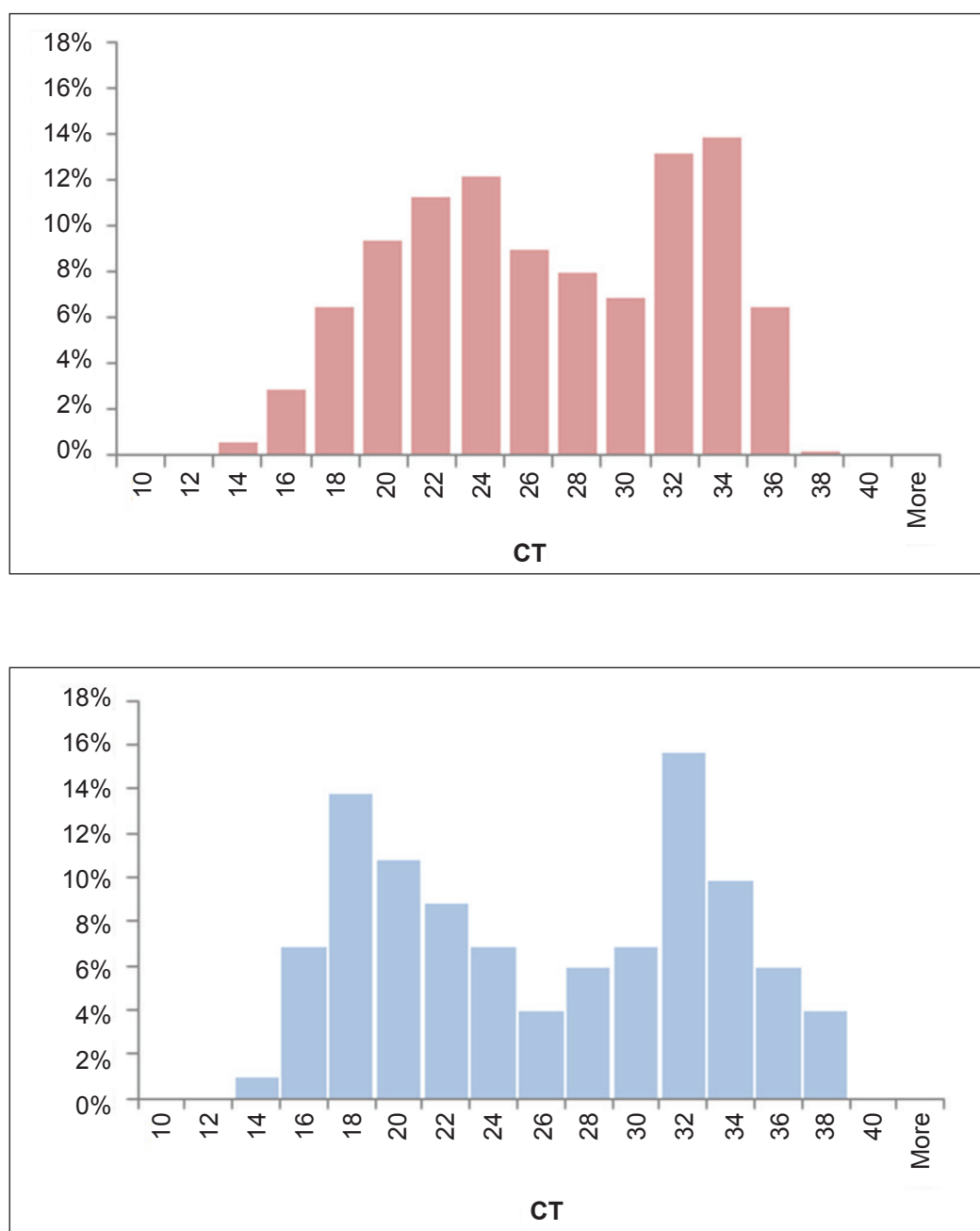
Figure 5. Distribution of cycle threshold (Ct) for N gene in Top: symptomatic individuals (N=526) and Bottom: asymptomatic individuals (N = 102).
