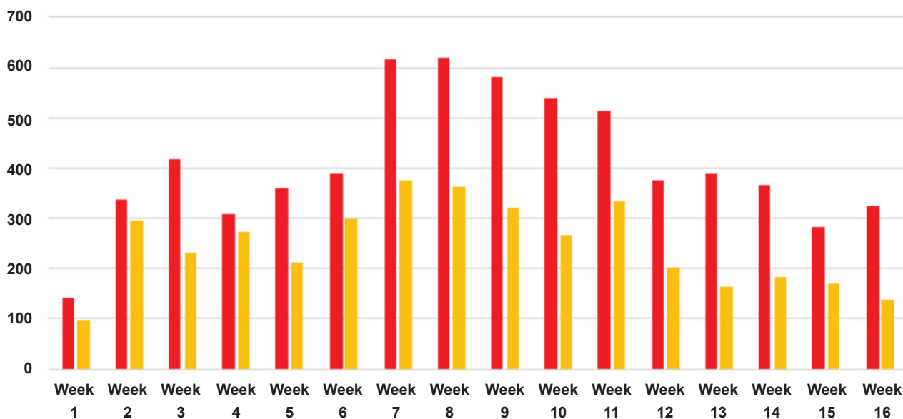
Figure 15. Number of suspected/confirmed (red) cases contacted and close contacts (orange) identified per week.
