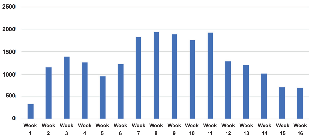
Figure 16. Number of follow-ups with close contacts per week.
