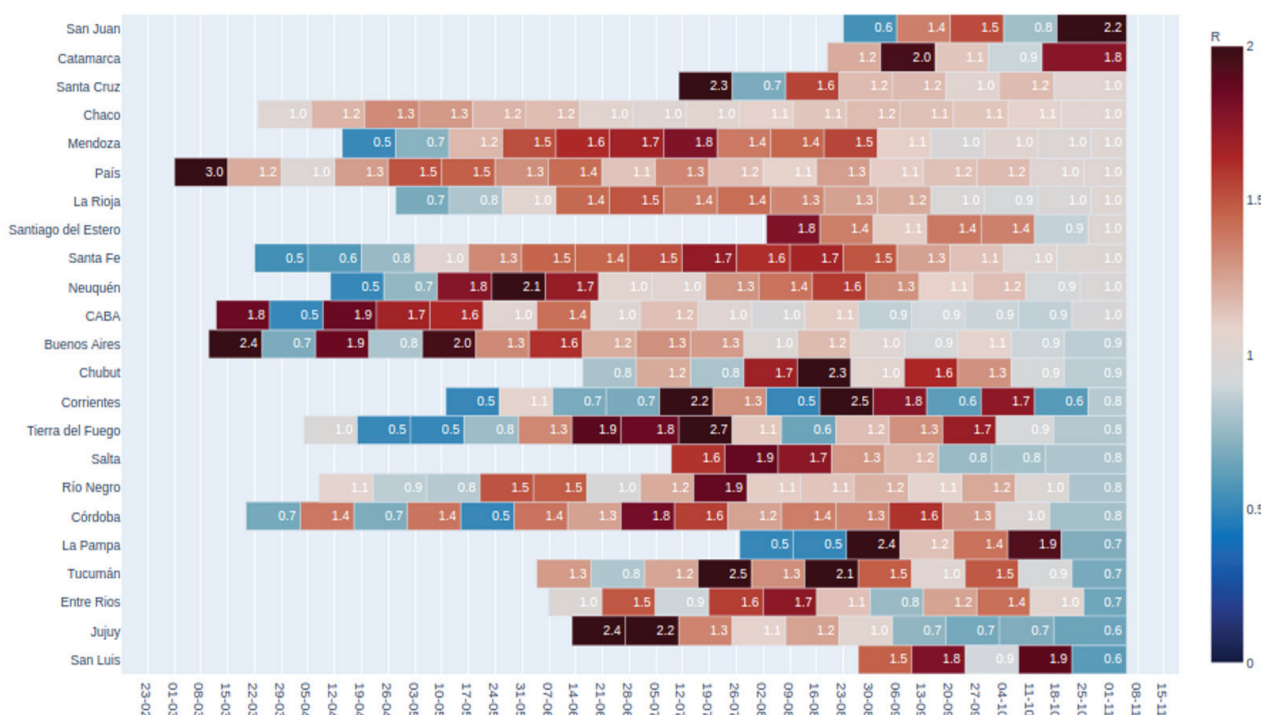
Figure 2. Temporal heat map showing evolutions of the effective reproductive number R_{eff}(t) for the Argentine provinces (snapshot of 11/15/2020). This display is part of the automated analysis available on the website described in Section 1.4.
